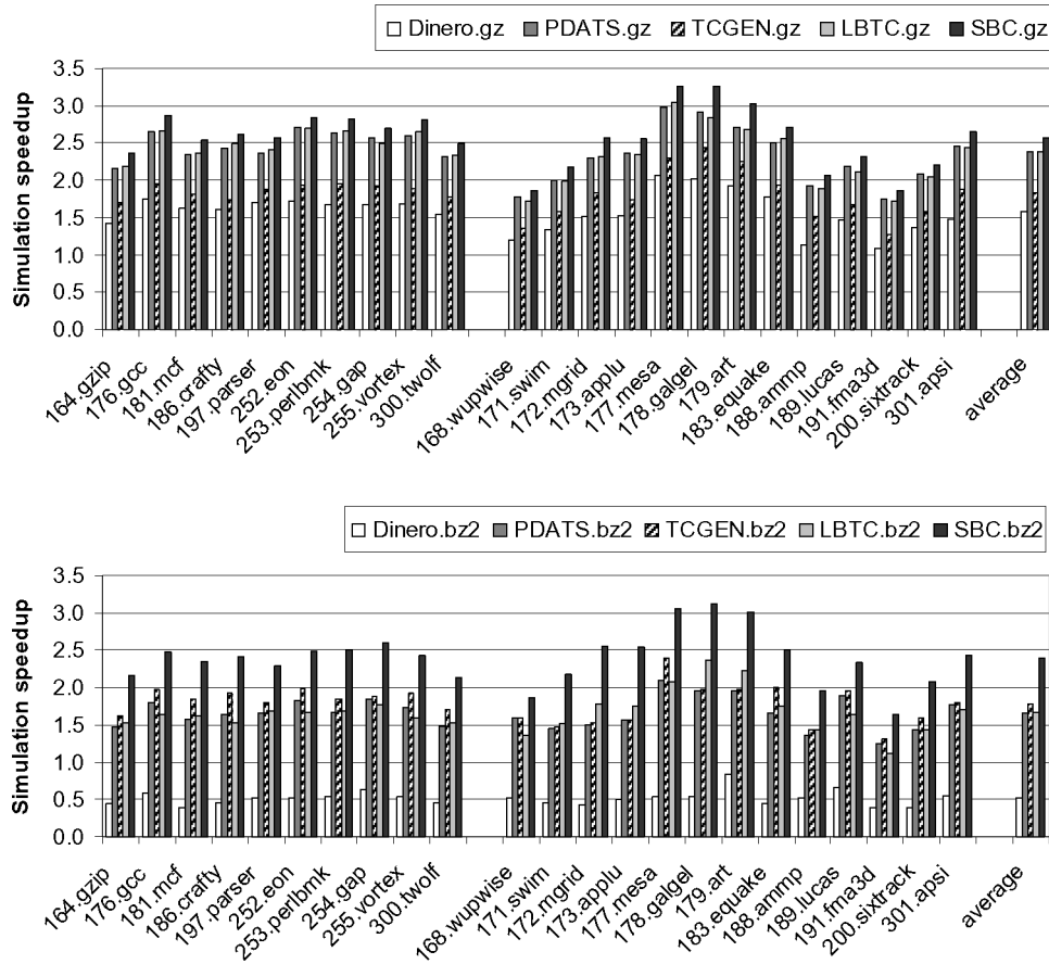
Fig. 11. Simulation speedup for the DineroIV simulator, relative to raw Dinero traces.
