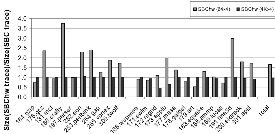
Fig. 13. SBChw versus SBC trace sizes.
