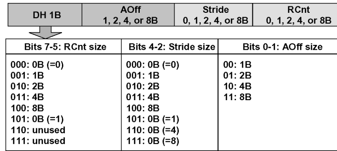
Fig. 4. Format of the SBC data trace.
