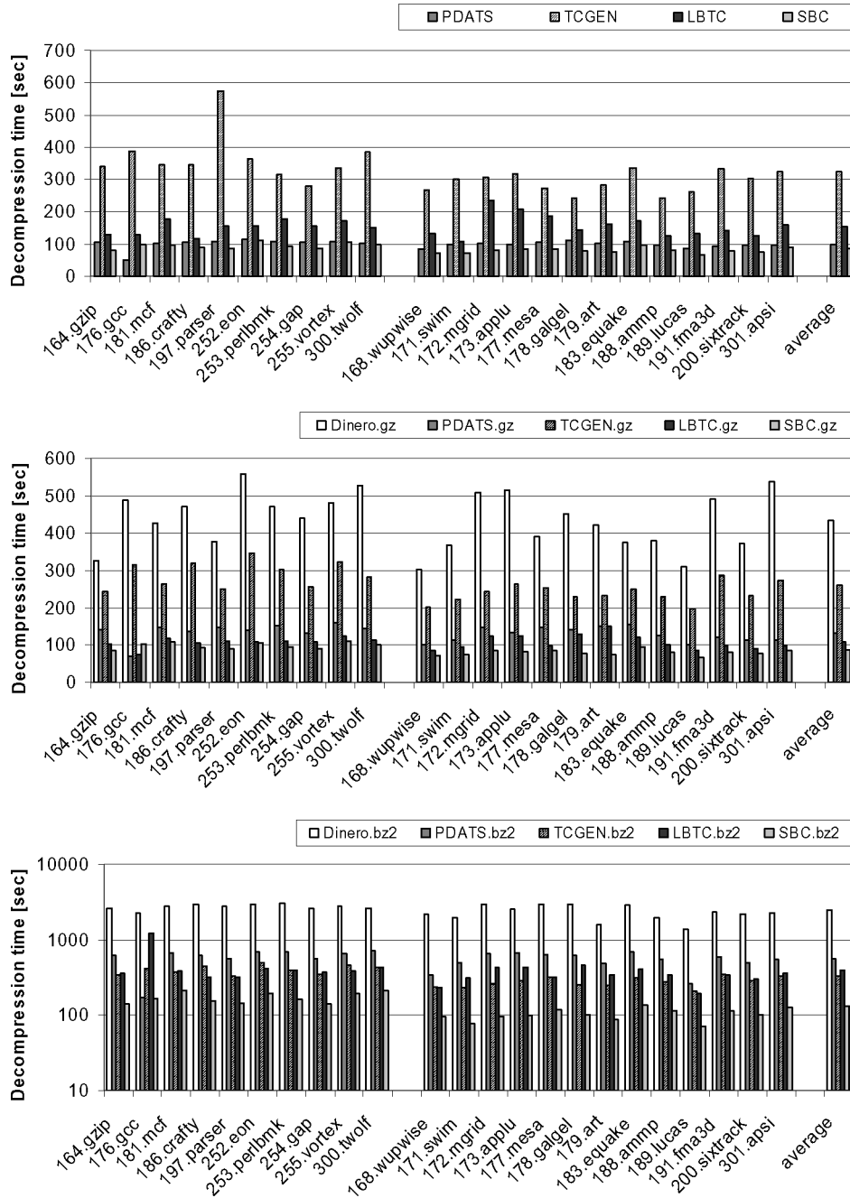
Fig. 10. Decompression time.
