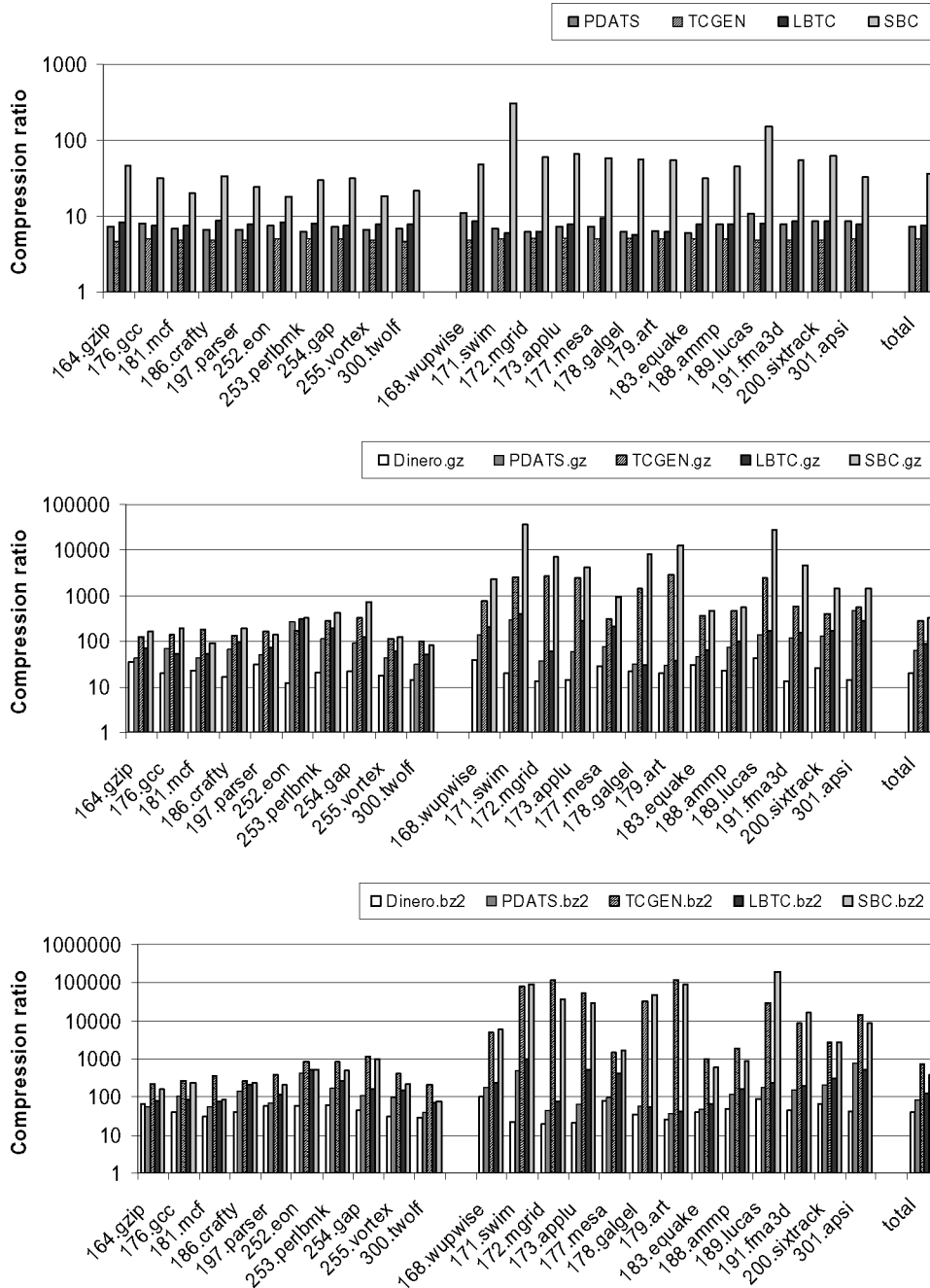
Fig. 9. Compression ratio.
